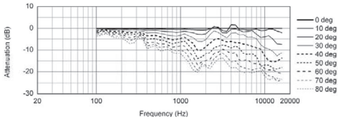
Horizontal Off-Axis Frequency Response
